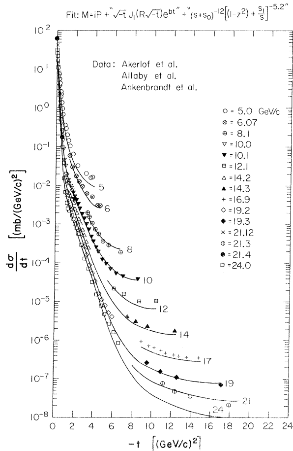
FIG. 10. A fit to the pp differential cross section when the forward Pomeranchukon exchange is included. The fit is constrained at large t, u to the asymptotic-interchange prediction d\sigma/dt \rightarrow Cs^{-12}(1-z^2)^{-5.2} .
