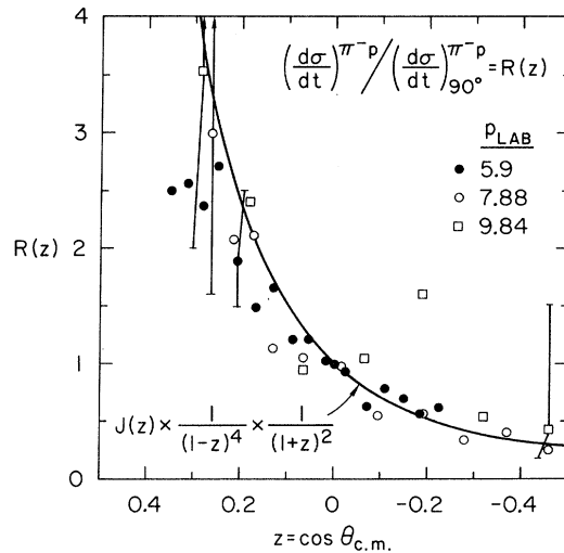
FIG. 7. The dependence of the \pi^-p differential cross section on z ( \cos \theta ) in the center-of-mass system. The lack of any strong energy dependence of the ratio should be noted. The solid line is our prediction given in Eq. (5.25) with \alpha=2\beta .
