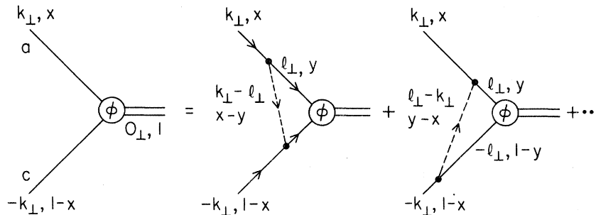
FIG. 4. An example of the lowest-order binding potential and the equation satisfied by the vertex function.
